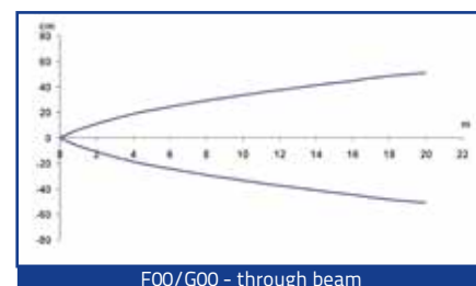
F00/G00 - through beam
